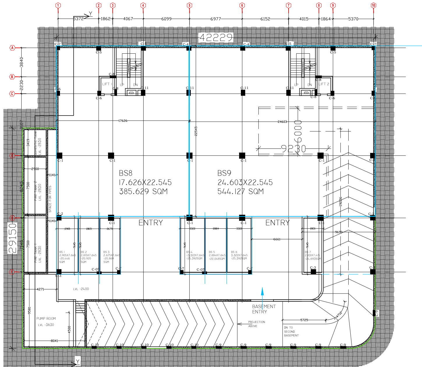
BASEMENT I
